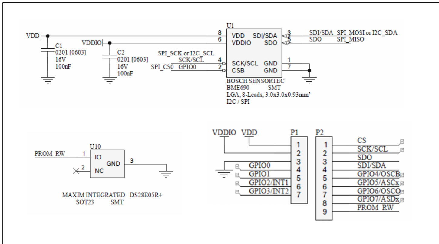
Electrical layout
